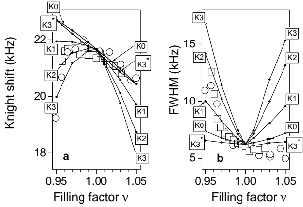
FIG. 5. Open symbols are [K_S(\nu), \Gamma_w(\nu)] data from Fig. 2c. Filled points are [K_S^{Sim}(\nu), \Gamma_w^{Sim}(\nu)] extracted from simulations described in the text. The points for each Skyrmion type are joined by lines.
